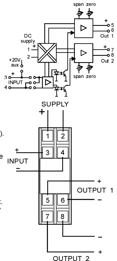
Block Diagram
